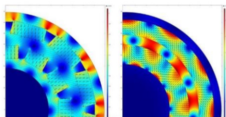
Figure 6: Flux path and magnetic flux density for a classical magnetic coupling and a powder-based magnetic coupling.
