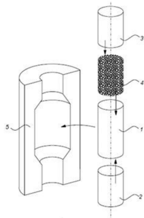
Figure 2: IP Magnet process.
