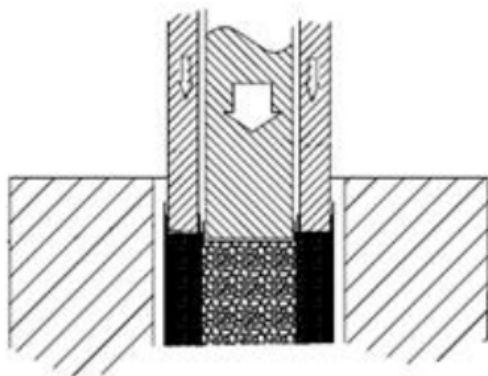
Figure 4: Compression of both iron powder and magnet powder in one process.
