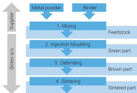
Figur 4: Illustration of the MIM process
